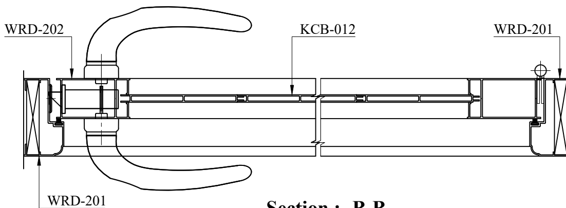
Section :- B-B
