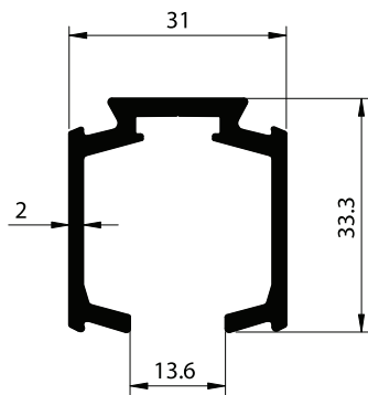
SECTION NO. - TSD-1001 EST. WEIGHT - 0.662 KG./M.
