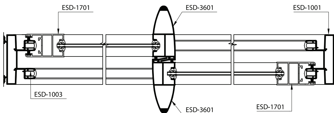
SECTION :- B-B
