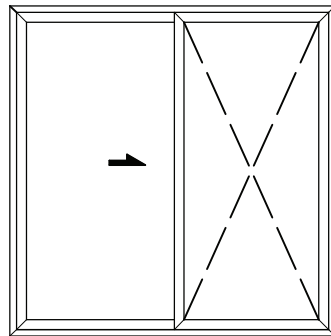
Sliding & Fixed
